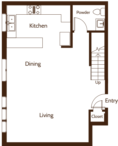
LEVEL ONE
